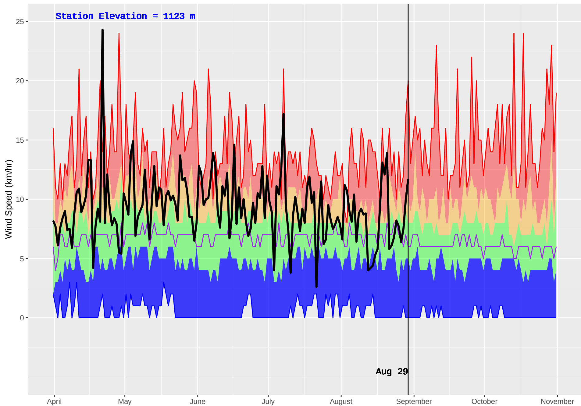
MCLEAN LAKE (311) : Historical (1987–2016) and Current (2018) Daily Wind Speed
